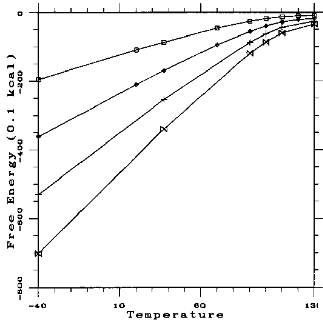
Fig. 3a, b. Average free energies as a function of temperature. a) AUGC alphabet (upper), b) GC alphabet (lower). \nu=20 \square , \nu=30 \circ , \nu=40 + , \nu=50 \triangleleft
