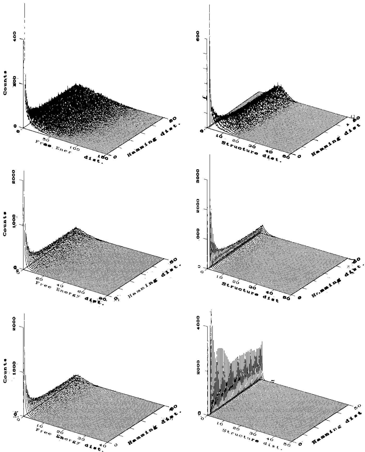
Fig. 9. Density surfaces \rho(\delta|d) for GCAU alphabet. a) Energy differences \delta = |F - F'| . b) Structure distance. top T = 37^\circ\text{C} , center T = 70^\circ\text{C} , bottom T = 100^\circ\text{C}
