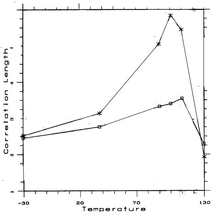
Fig. 8. Structure correlation length a) GCAU alphabet (upper), b) GC alphabet (lower). n = 30 \square , n = 50 \star
