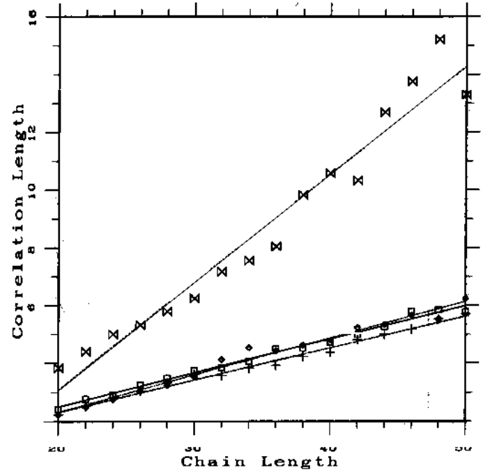
Fig. 5a, b. The correlation length is plotted versus the chain length. Straight lines are least square fits to the computed data. a) GCAU alphabet (upper): T=-30^{\circ}\text{C} \square , solid line. T=37^{\circ}\text{C} \diamond , dotted line. T=70^{\circ}\text{C} + , dash-dotted line. T=100^{\circ}\text{C} \triangle , dashed line. b) GC alphabet (lower): T=-40^{\circ}\text{C} \square , solid line. T=37^{\circ}\text{C} \diamond , dotted line. T=100^{\circ}\text{C} + , dash-dotted line. T=130^{\circ}\text{C} \triangle , dashed line. Owing to computer time limitations the data for the \nu \geq 30 , have been sampled with smaller precision as for shorter chain length
