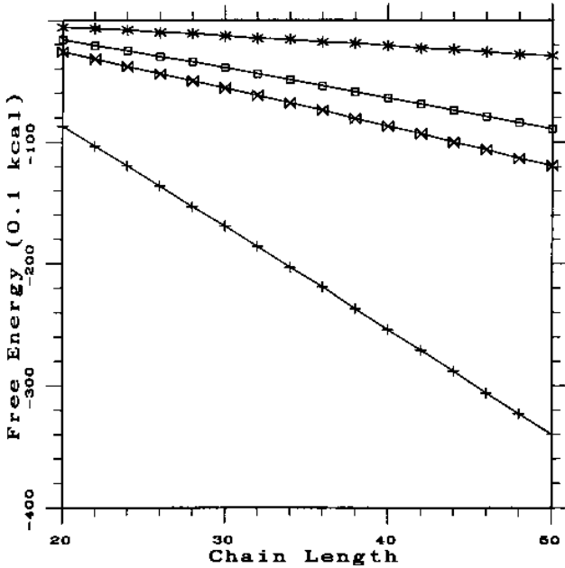
Fig. 2. Average free energies as a function of the chain length. For both the GCAU and the GC alphabet two different temperatures are shown. (GCAU: T=37^{\circ}\text{C} \square , T=70^{\circ}\text{C} \star , GC: T=37^{\circ}\text{C} + , T=90^{\circ}\text{C} \triangleleft )
