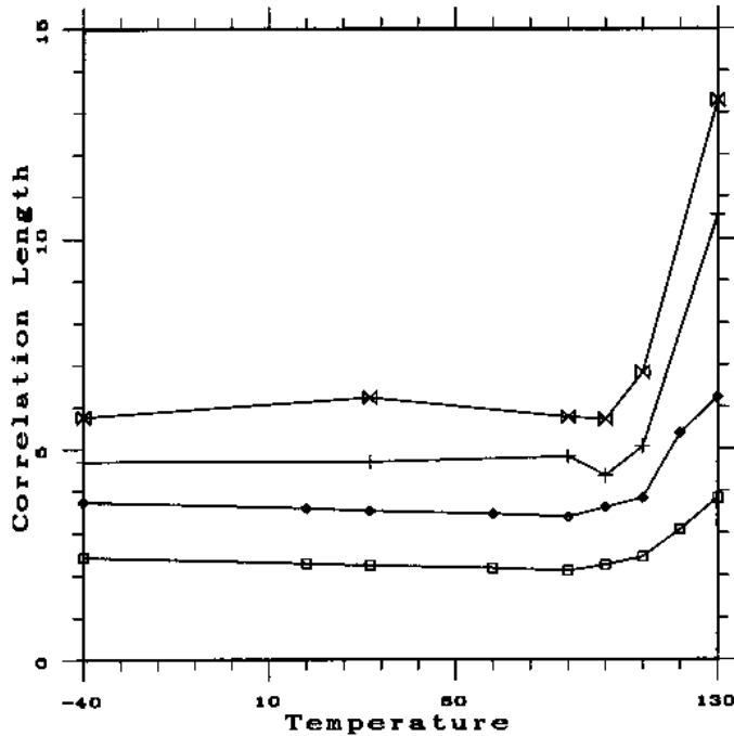
Fig. 6a, b. Temperature dependence of the free energy correlation length. a) GCAU alphabet (upper), b) GC alphabet (lower). v=20 \square , v=30 \diamond , v=40 + , v=50 \times . The critical temperatures are T_c \approx 70^\circ\text{C} for the GCAU alphabet, T_c \approx 100^\circ\text{C} for the GC alphabet, respectively
