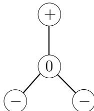
Fig. 2. This second eigenvector has 3 strong sign graphs.
