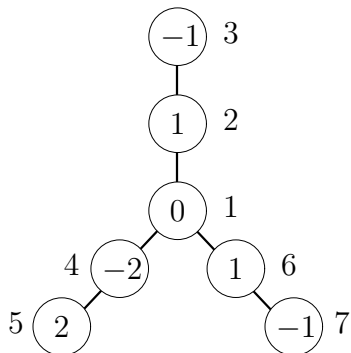
Fig. 1. The eigenvector corresponding to \lambda_5 has 6 strong sign graphs.
