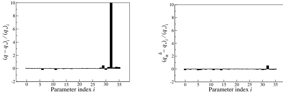
Figure 20. Individual relative errors of the identified parameters. Left: solution \tilde{q} obtained via pure minimization of the data mismatch, i.e. without regularization. The relative error of parameter 32 is 3085.45 (not shown here due to the cut-off at 10). Right: solution q_\alpha^\delta obtained via Tikhonov regularization.
